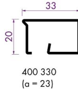
Aluminium glaslat 33x20mm
