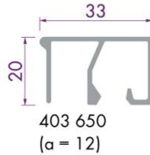
Aluminium glaslat 33x20mm
