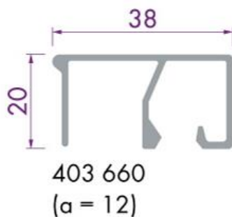
Aluminium glaslat 38x20mm
