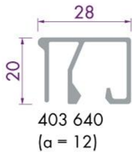
Aluminium glaslat 28x20mm
