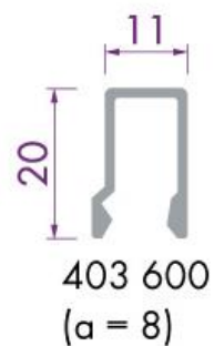
Aluminium glaslat 11x20mm
