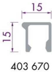
Aluminium glaslat 15x15mm
