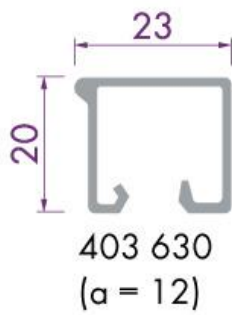
Aluminium glaslat 23x20mm
