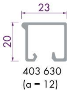
Aluminium glaslat 23x20mm
