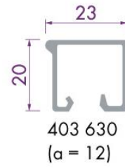
Aluminium glaslat 23x20mm
