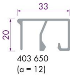
Aluminium glaslat 33x20mm
