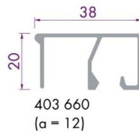
Aluminium glaslat 38x20mm
